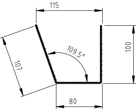
SECTION E-E SCALE 1:4
